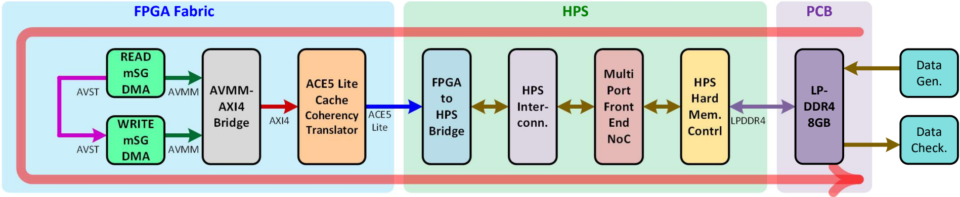
SpaceBridge Custom Loopback based on mSG-DMA Example Design
