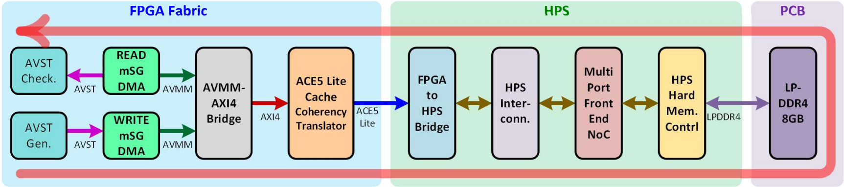
Critical Link mSG-DMA Example Design
